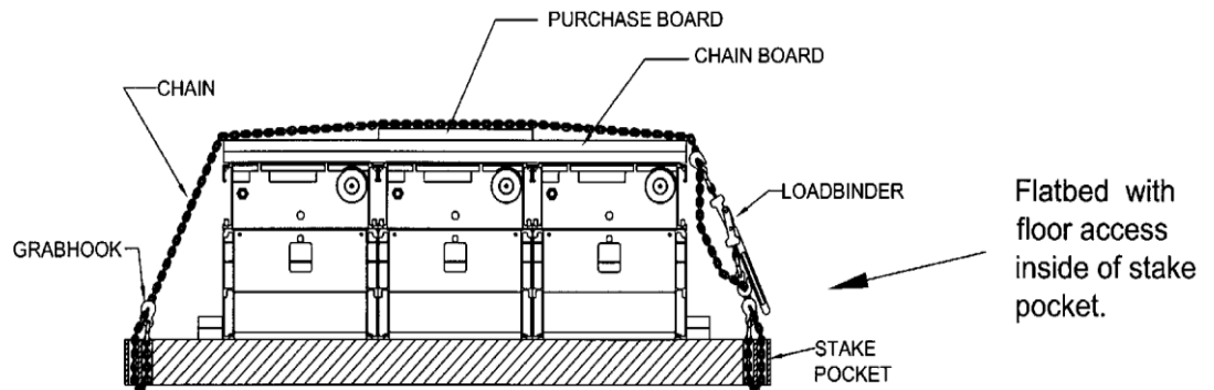
FIGURE B-13. Typical tiedown using chain and loadbinder.
